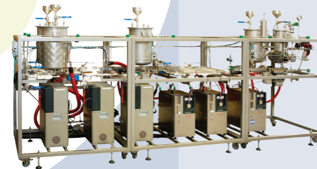
Dosing and reaction unit for dosing various fluids
